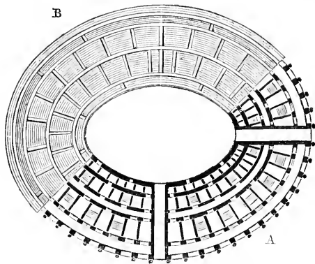
Fig. 19. Ground-plan of an amphitheatre.
